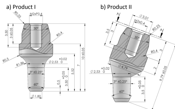
Figure 1. Dimensions and tolerances of the products
