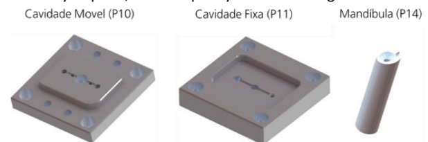
Figure 2. 3D design of the micro mold with cavities
