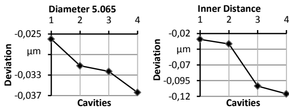
Figure 3. Dimension deviations for sequentially produced cavities
